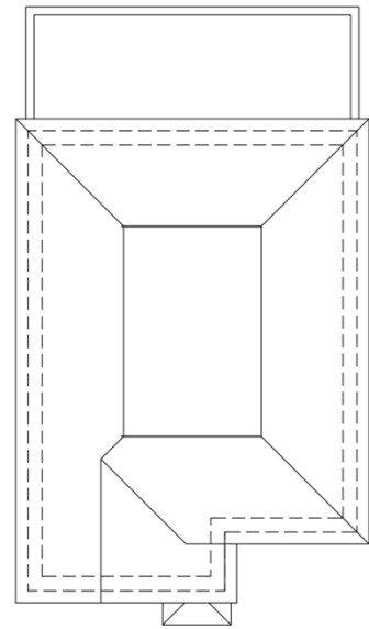
Roof Plan
